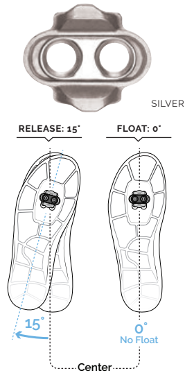
STANDARD RELEASE 0° FLOAT CLEAT
