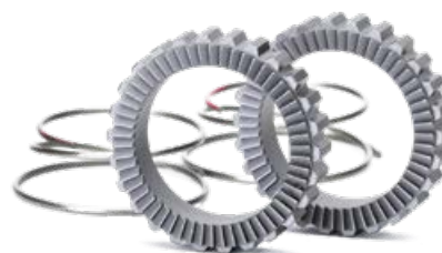
RATCHET HUBS 6.6° ENGAGEMENT UPGRADE KIT UPGRADES RATCHED HUBS ENGAGEMENT FROM 10 TO 6 DEGREES
