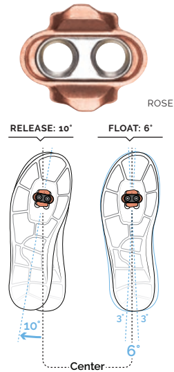
EASY RELEASE 6° FLOAT CLEAT
